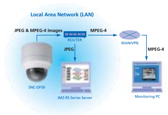
Dual Image Encoding
