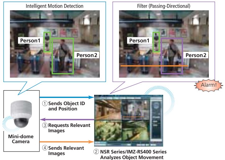
Distributed Enhanced Processing Architecture (DEPA)
